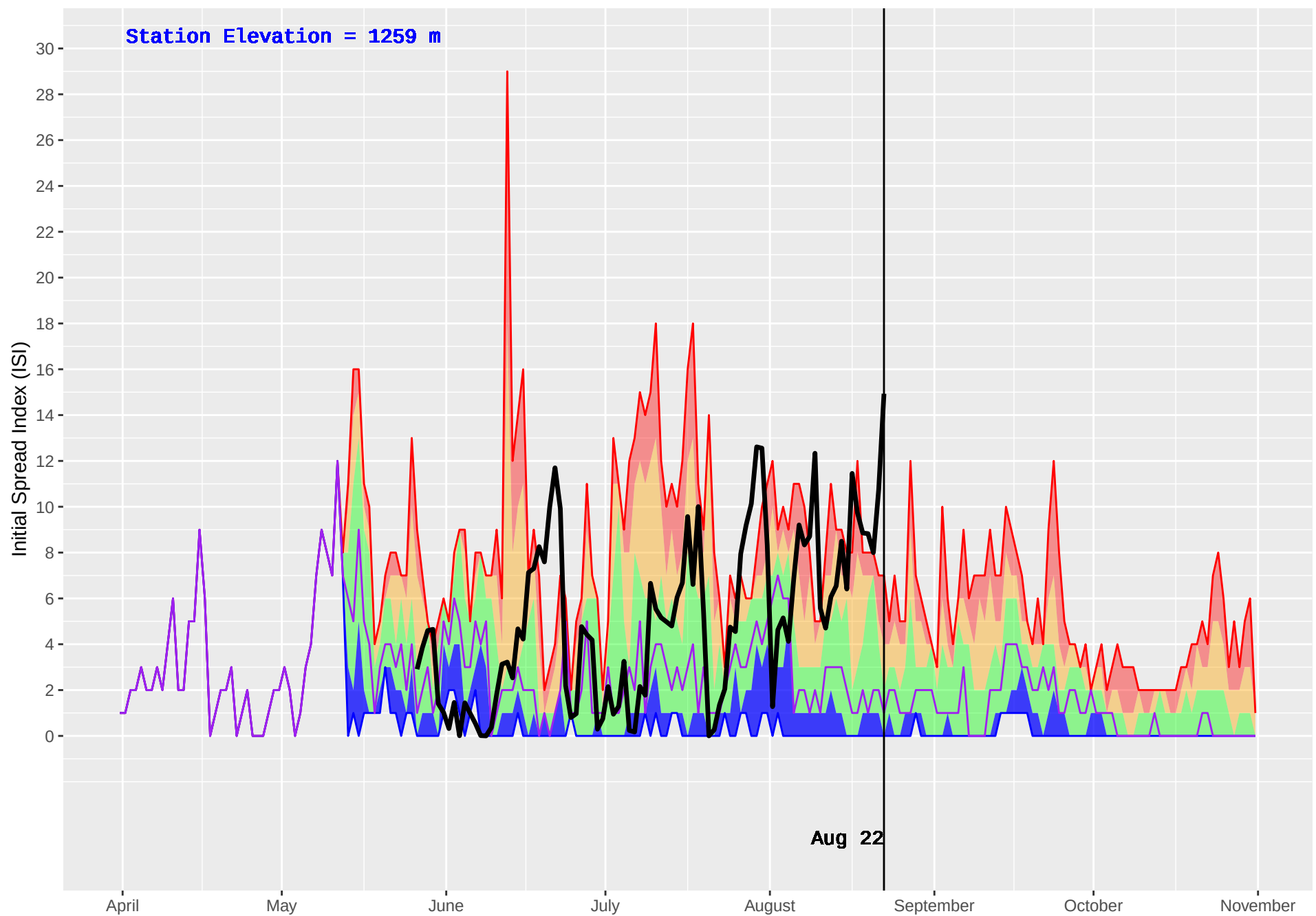
PARROTT (183) : Historical (1995–2016) and Current (2018) Daily Initial Spread Index (ISI)
