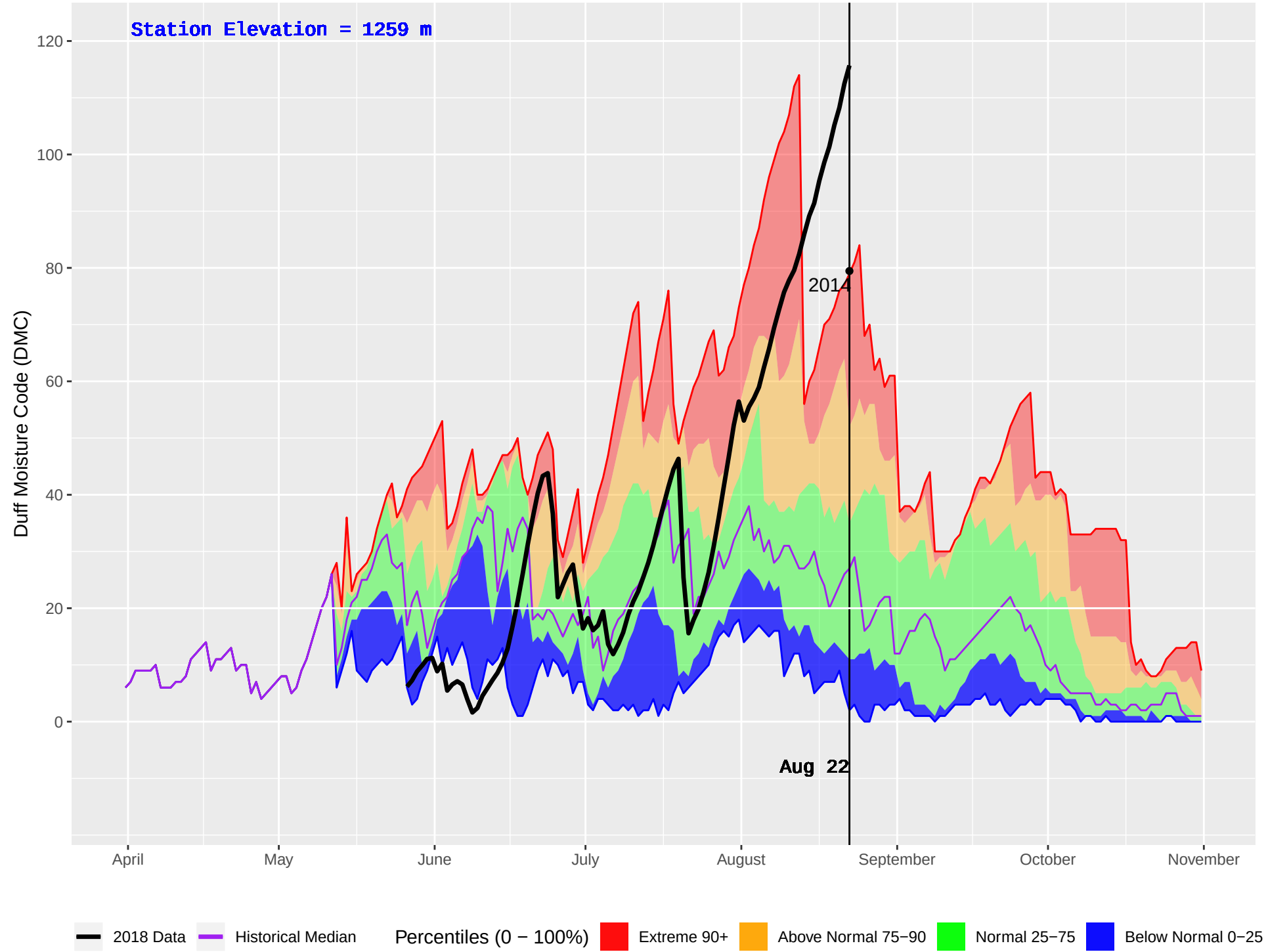
PARROTT (183) : Historical (1995–2016) and Current (2018) Daily Duff Moisture Code (DMC)
